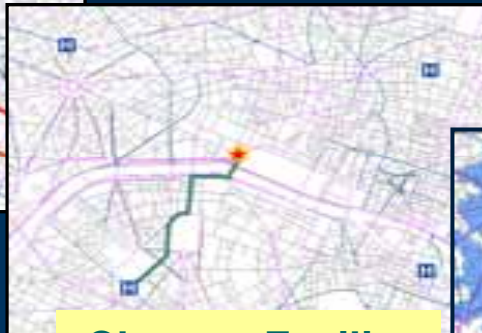
Closest Facility
