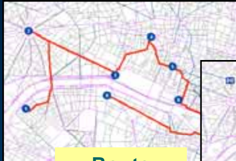
Route
