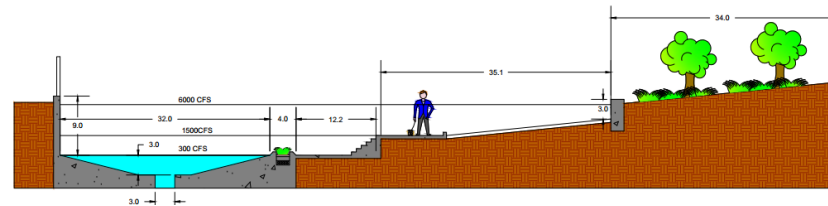
SECTION C-C
