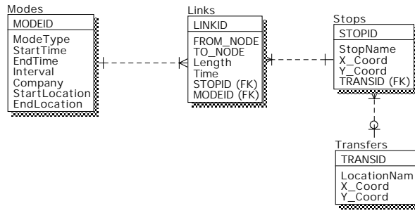
Figure 5. ERD for GIS Data Construction
