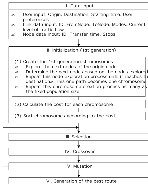
Figure 3. Flow of the GA process
