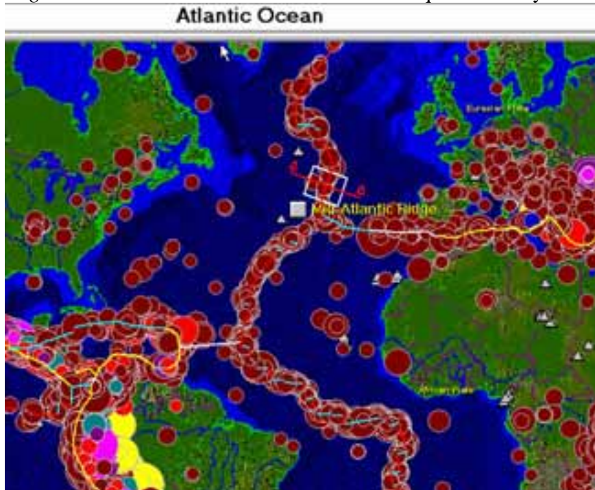
Figure 4. Plate boundaries and simulated earthquake activity
