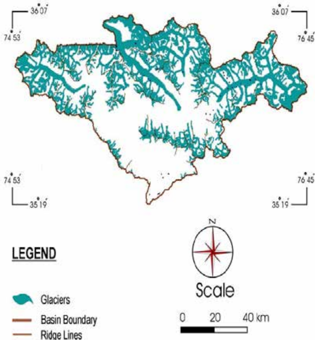
Figure 4.21: The glacier distribution in the Shigar river basin showing Baltoro and Biafo glaciers significance in the region being the largest.
