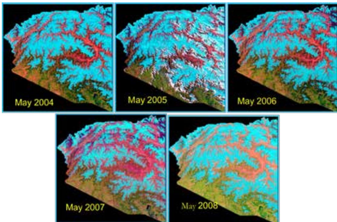
Figure 4.3: Depletion of Glaciers in Pakistan from 2004 – 2008.
