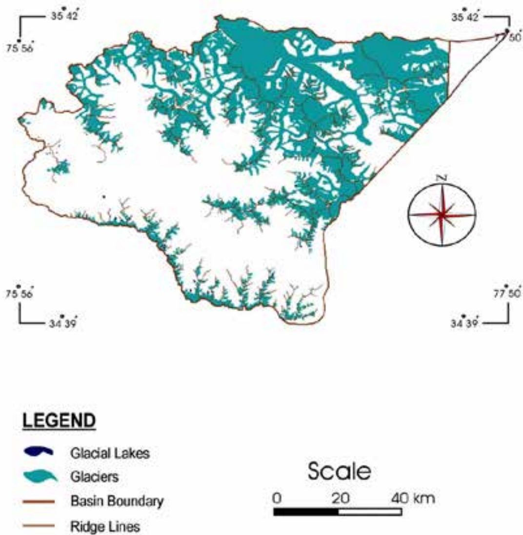
Figure 4.4 : The Glaciers Distribution in Shyok River basin.
