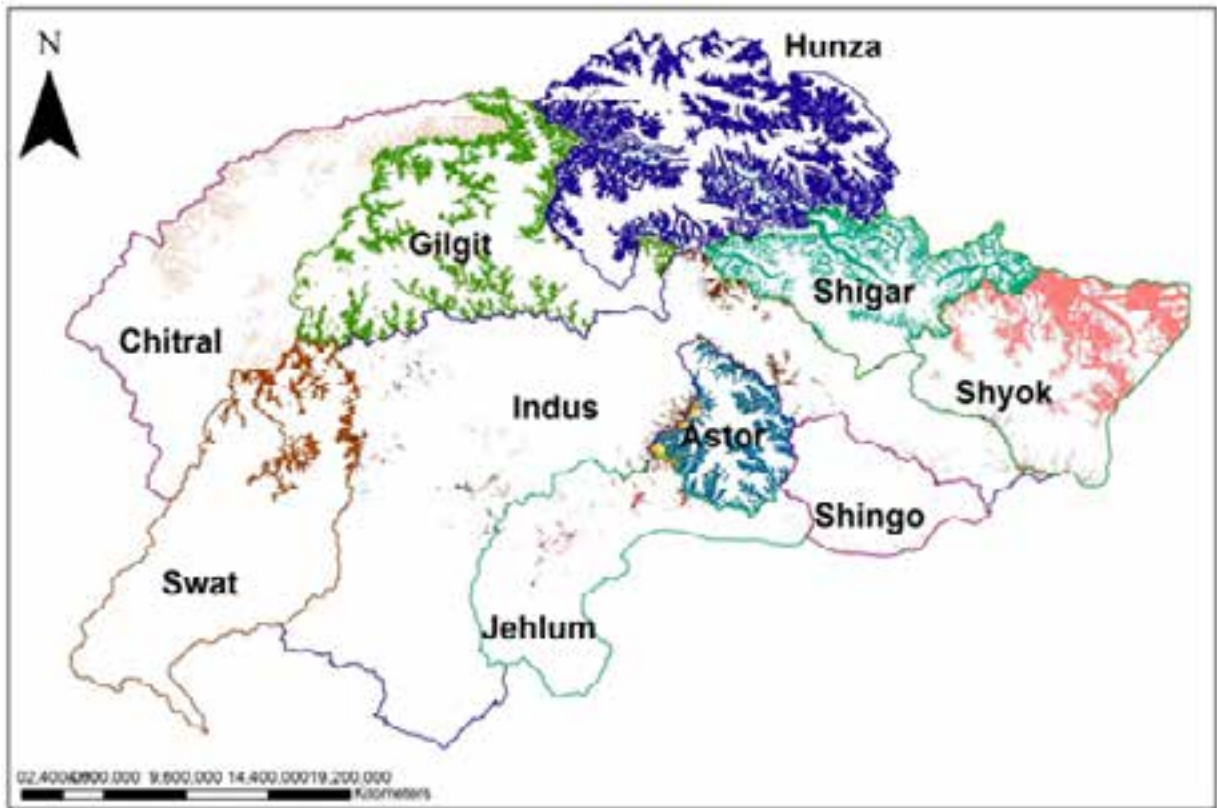
Figure 3.1: Distribution of Glaciers in 10 River Basins of Northern Pakistan
