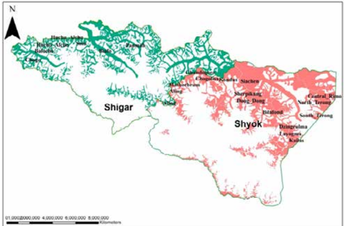
Figure 1.2: The Distribution of glaciers in Shigar and Shyok basins.
