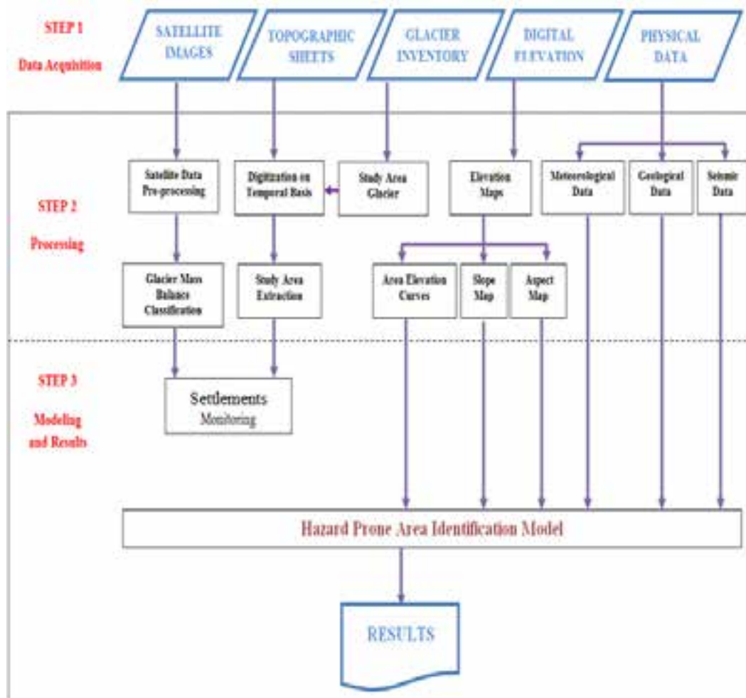
Figure 3.2: Methodological Flow Chart of Geospatial Analysis of Glacial Hazard.
