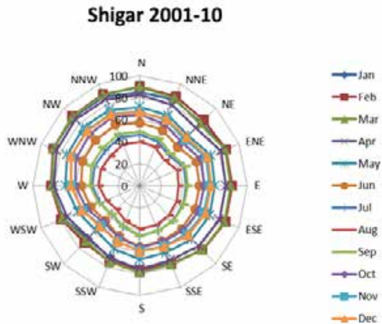
Figure 4.22: Aspect Wise Snow Coverage in Km of Shigar Basin
