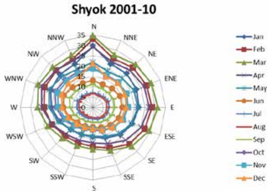
Figure 4.7: Aspect Wise Snow Coverage in Km of Shayok Basin
